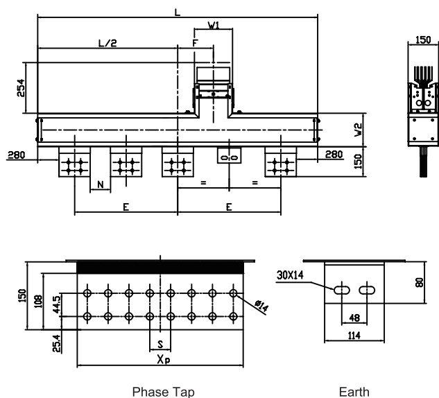
Overall dimensions
