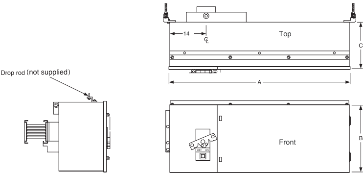
Figure3: 630-1000A plug-in unit
