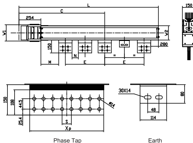
Overall dimensions
