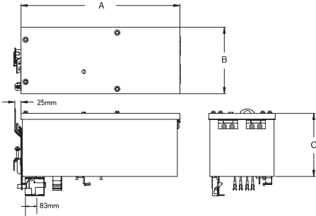
Figure1: 16-250A plug-in unit
